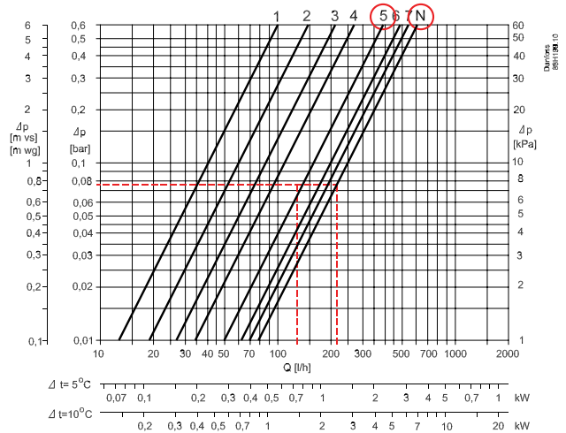
Manifold with flowmeter
