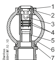
Supply manifold without flowmeter
