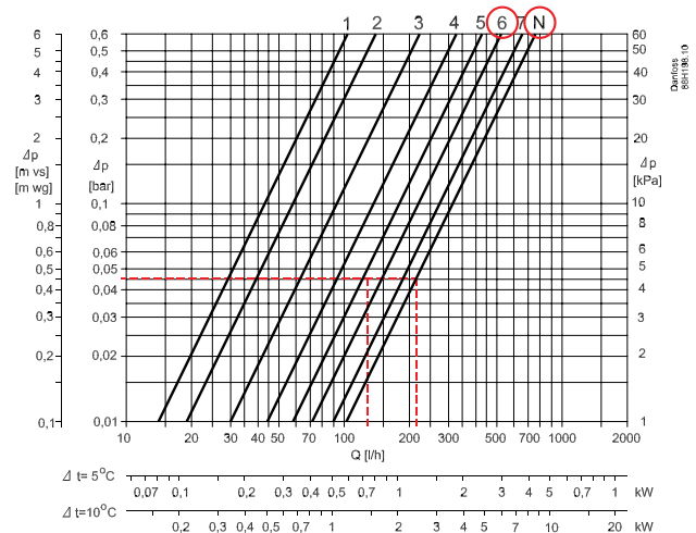
Manifold without flowmeter
