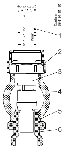
Supply manifold with flowmeter
