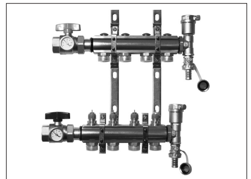
Manifold without flowmeter
