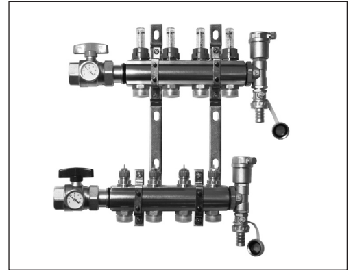
Manifold with flowmeter
