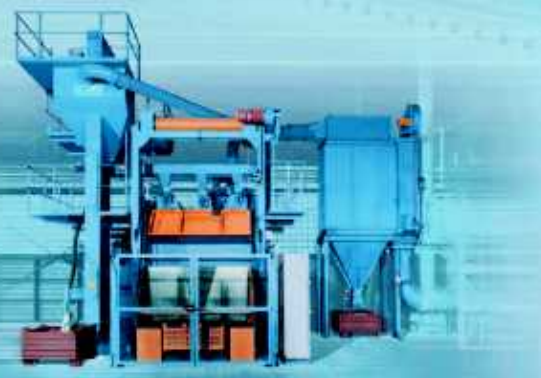
Polygonal shot blast machine DTC 3
